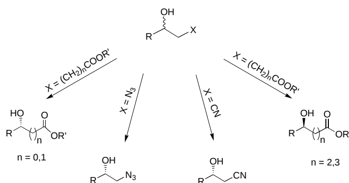
Scheme 1. Dynamic kinetic resolution of functionalized alcohols with efficient use of all racemate.
