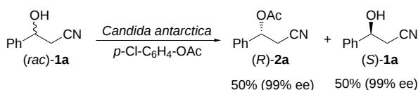
Scheme 6. Lipase-catalyzed transesterification of \beta -hydroxy nitrile 1a .
